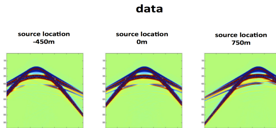
Figure 2: pre-stack data
