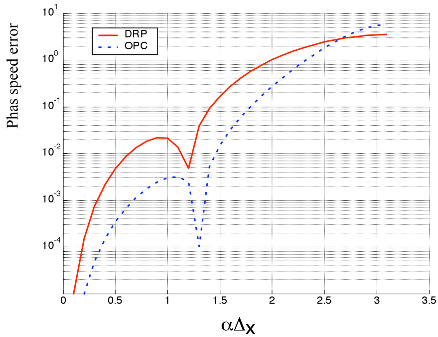
Figure 4. Phase speed error on a logarithmic scale
