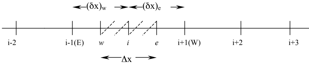
Figure 1 Grid points cluster for one-dimensional problem
