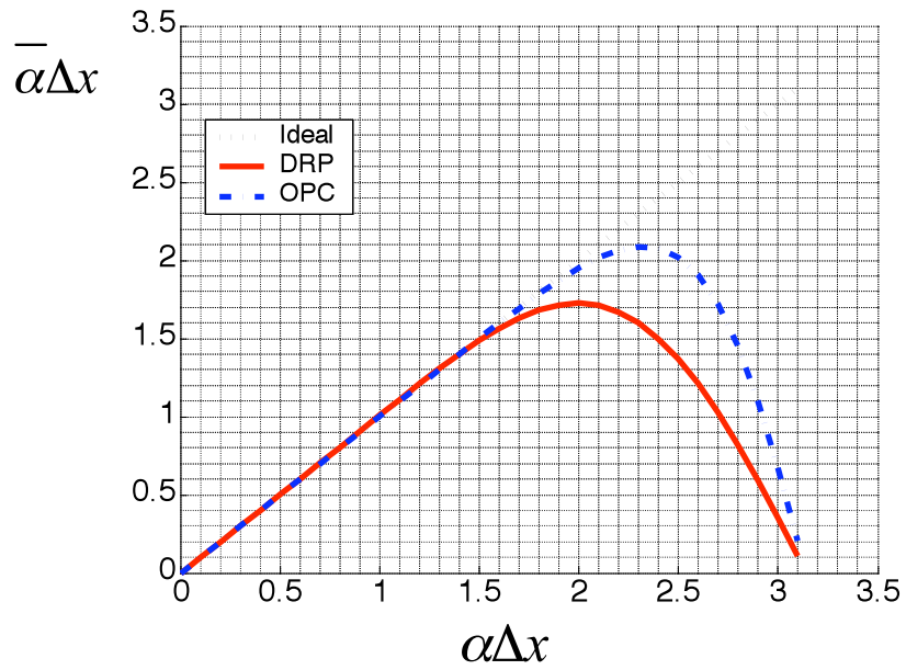
Figure 3. Dispersive characteristics of the schemes
