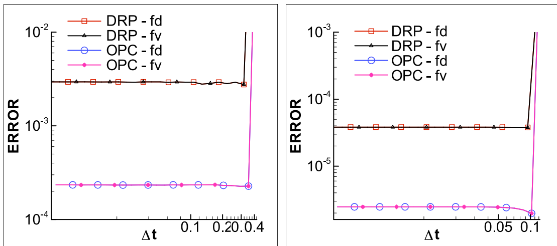
Figure 6. Errors with respect to the time step size under a fixed space \Delta x , at t=50 - linear wave equation
