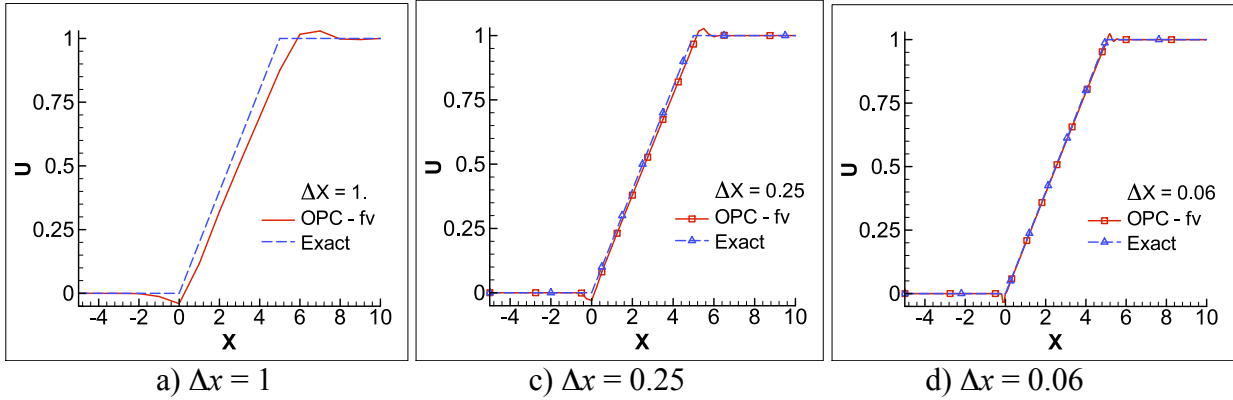
Figure 12. OPC-fv solution - nonlinear wave equation; t = 5 ; CFL=0.5
