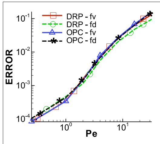
Figure 13. Error in function of Pe - nonlinear Burgers equation; \Delta x = 0.25 ; CFL=0.2 ; t = 20
