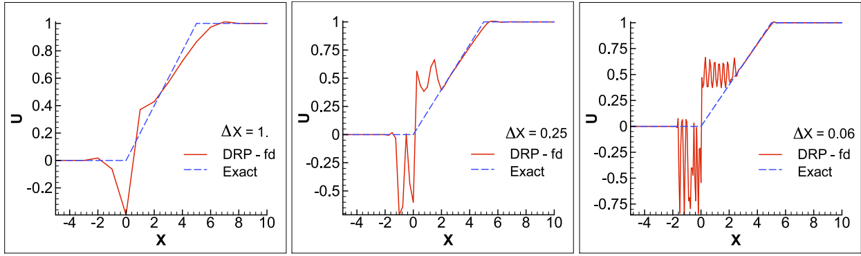
a) -\Delta x = 1 b) -\Delta x = 0.25 c) \Delta x = 0.06 Figure 9. DRP-fd solution - nonlinear wave equation; t = 5 ; CFL=0.5
