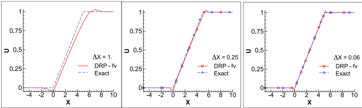
a) x = 1 b) -\Delta x = 0.25 c) \Delta x = 0.06 Figure 10. DRP-fv solution - nonlinear wave equation; t = 3 ; CFL=0.5
