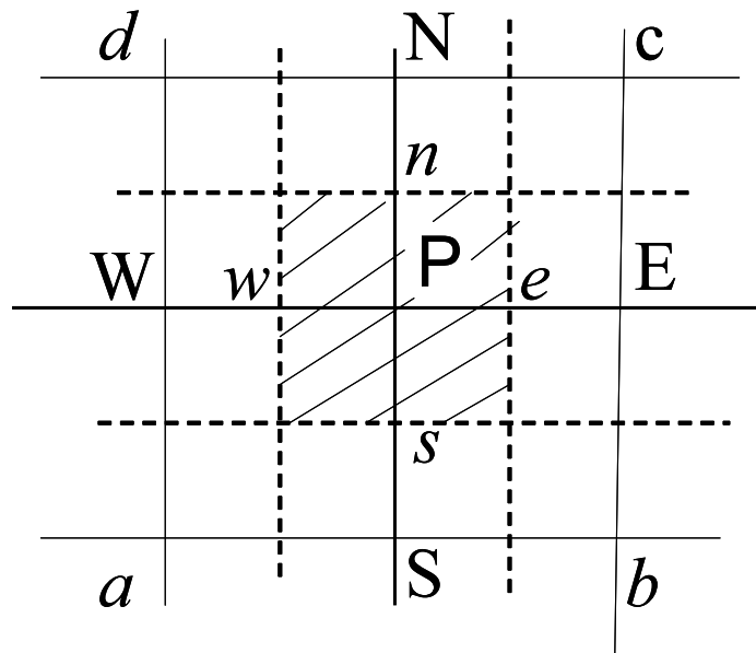
Figure 2 Grid notation for two-dimensional problem, where (i) P denotes the center of a cell, (ii) E, W, N, and S denote, respectively, the nodes corresponding to the east, west, north and south neighbors, (iii) e, w, n and s denote, respectively, the center of the east, west, north and south face of the cell, and (iv) a, b, c, and d denote, respectively, the corners of the cell
