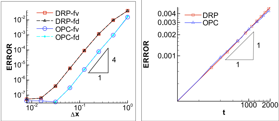
Figure 7. Errors under a fixed CFL = 0.5, at t=50 - linear wave equation: a) error with respect to the space size; b) accumulation of the error in time
