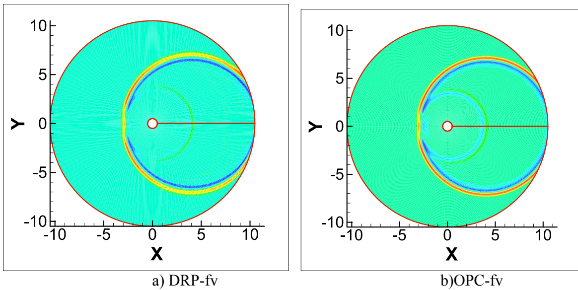
Figure 16. Instantaneous pressure contours at time t = 7 – two-dimensional acoustic scattering problem
