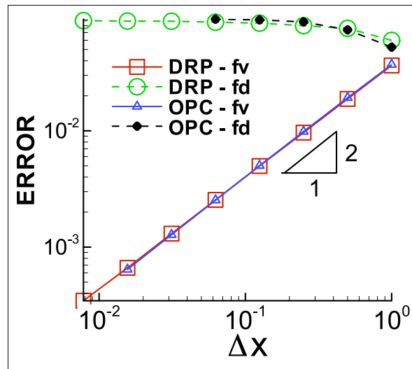
Figure 8. Errors with respect to the space step size under a fixed CFL = 0.5, at t=5 , - nonlinear wave equation
