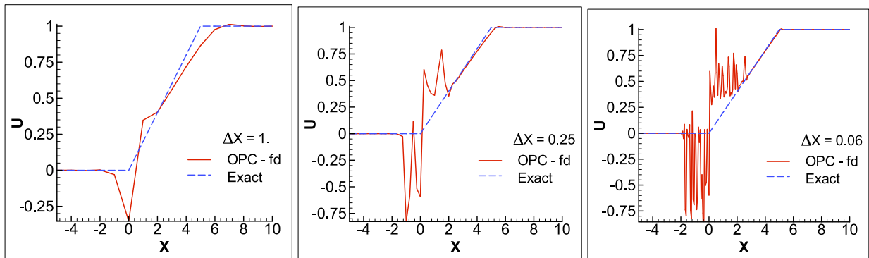
a) \Delta x = 1 b) \Delta x = 0.25 c) \Delta x = 0.06 Figure 11. OPC-fd solution - nonlinear wave equation; t = 5 ; CFL=0.5
