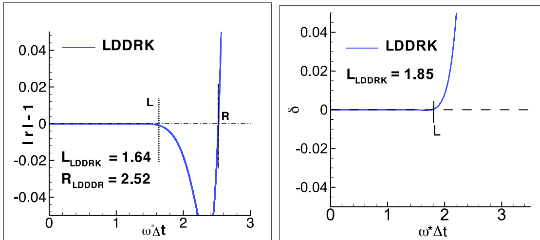
Figure 5 Four-stage optimized Runge-Kutta of order four scheme: a) dissipation error; b) phase error
