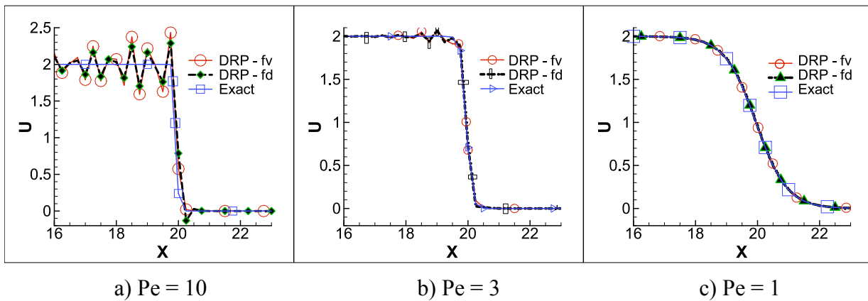
Figure 14. Numerical solution obtained by DRP schemes - nonlinear Burgers equation; \Delta x = 0.25 ; CFL=0.2 ; t = 20
